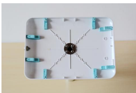
Place acrylic face sheet
