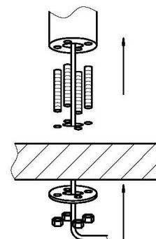
Mount from below surface
