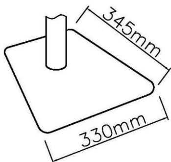
Floor stand with freestanding base
